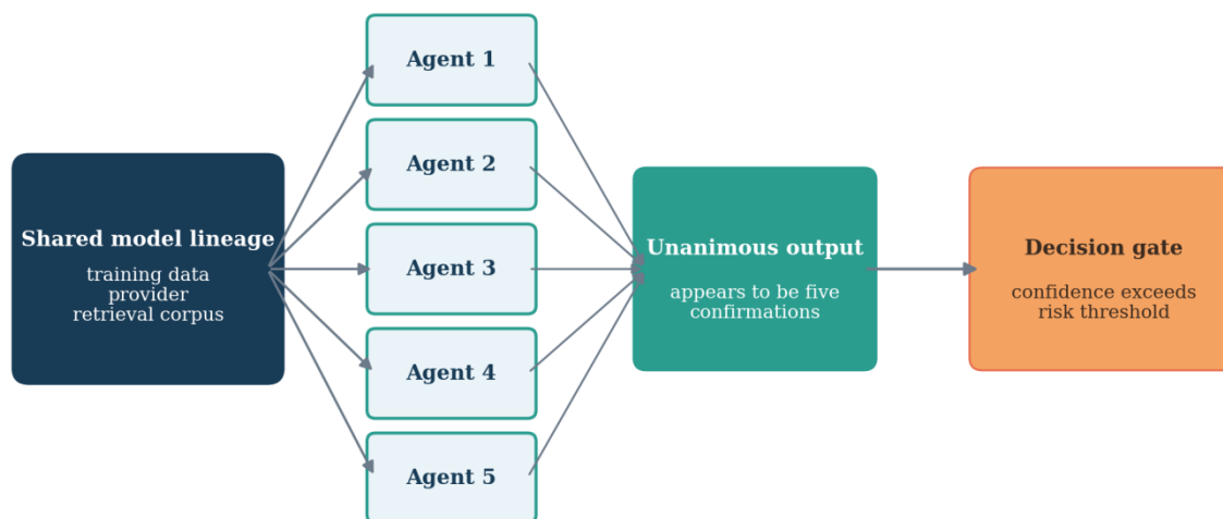
Hidden dependence converts repeated output into apparent evidence
