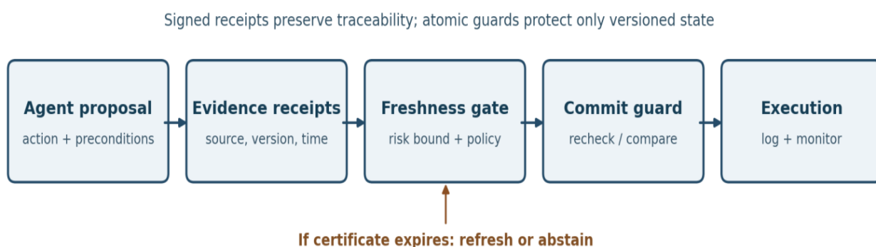
Figure 1. Reference architecture for freshness-aware tool execution. The abort or refresh branch is mandatory when the admissible certificate cannot be established.
