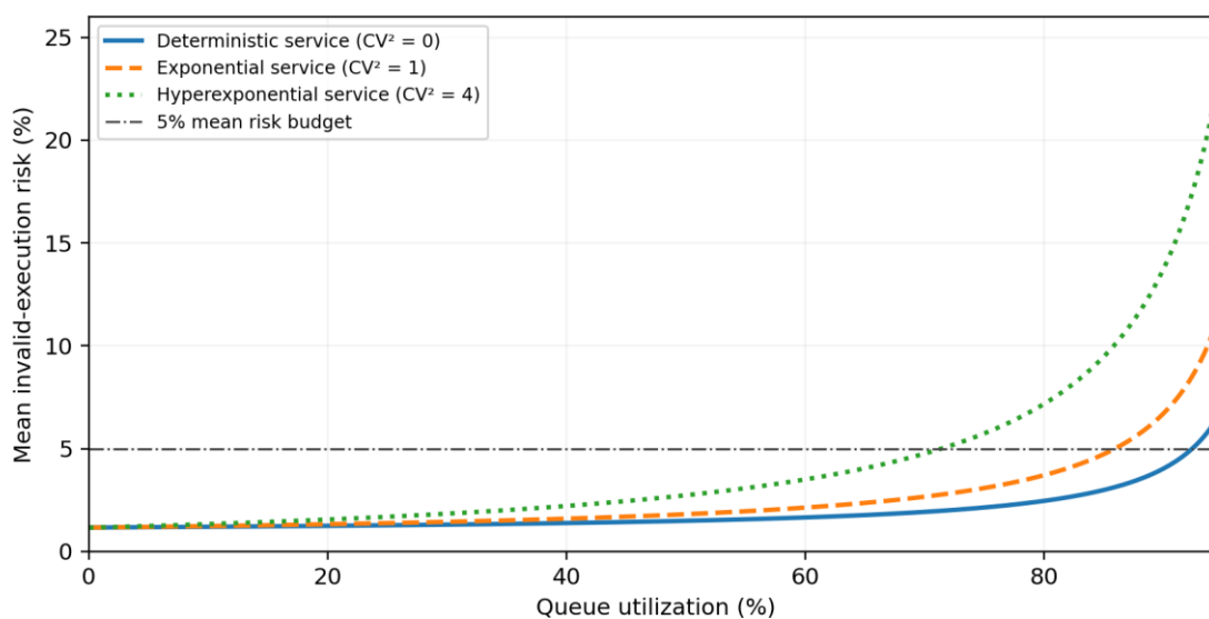
Figure 3. Exact mean risk from the M/G/1 transform across utilization and three service-time distributions. Unlike Figure 2, which changes only hazard, this figure varies service-time dispersion while fixing its mean.
