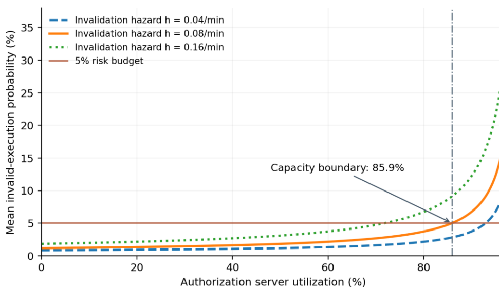
Figure 2. Analytical mean invalid-execution probability as authorization utilization increases, for three assumed hazards. The vertical marker shows the capacity boundary under the middle hazard and a 5% budget.
